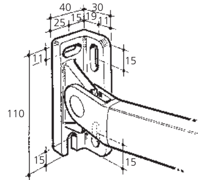
CHAPPE DE BRAS A RESSORT
